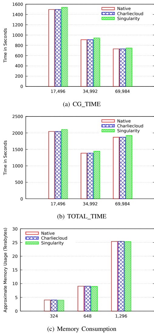
Fig. 2. Performance of Singularity, and Charliecloud containers against default run with MILC application at up to 70K processes
